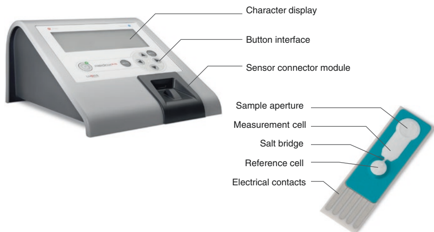
Fig. 3.2 Image of the portable RedoxSYS analyzer and disposable strip. From [36] with permission
